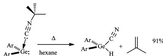
Scheme 1. C–H Bond Activation of tert -Butyl Isocyanide by Diarylgermylene
