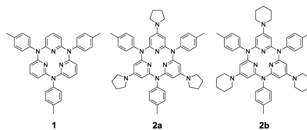
Figure 1. Azacalix[3](2,6)pyridine derivatives.
