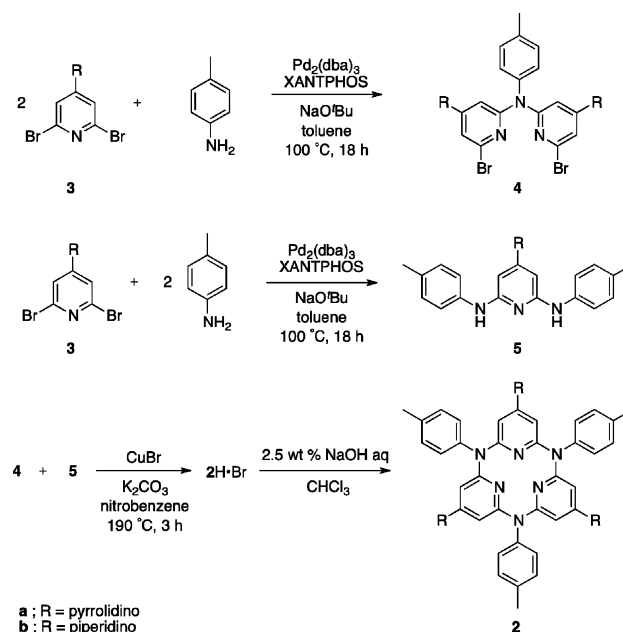
Scheme 1. Synthesis of 2
