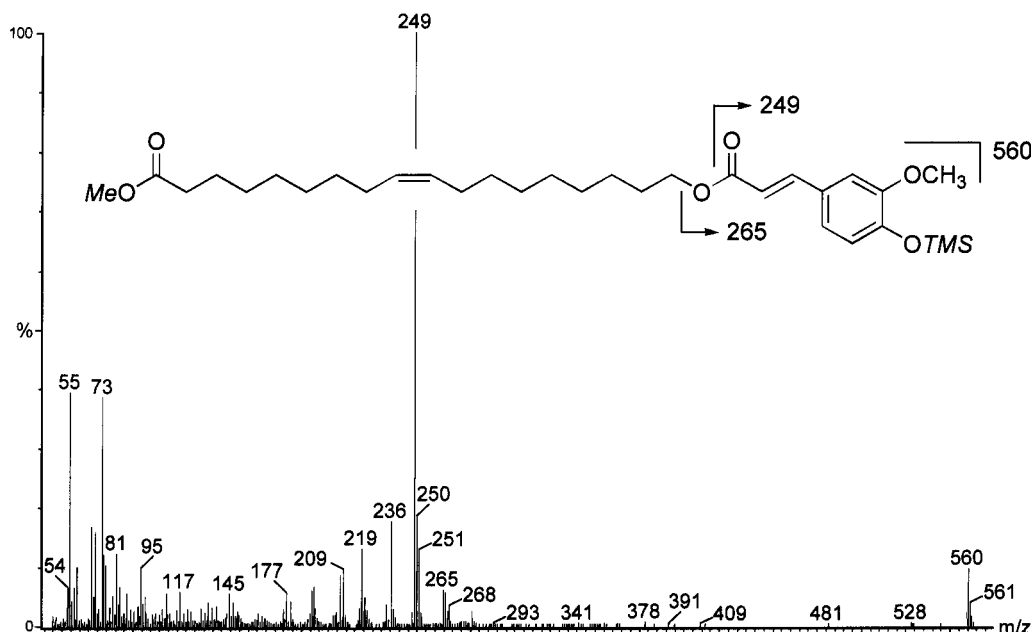
Figure 3. EI mass spectrum of the 18- O -feruloyloxyoctadec-9-enoic acid, methyl ester, trimethylsilyl ether, isolated from the \text{Ca}(\text{OH})_2 -catalyzed partial methanolysis products of the potato periderm suberin.
