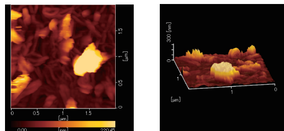
Figure 3. Surface morphology of film of 1 deposited onto HMDS-treated \text{Si}/\text{SiO}_2 at T_{\text{sub}} = 100^{\circ}\text{C} .
