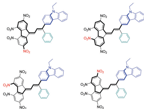
Fig. 4 Different mesomeric forms supporting the presence of two ICT bands for the TNF-based dye N .
