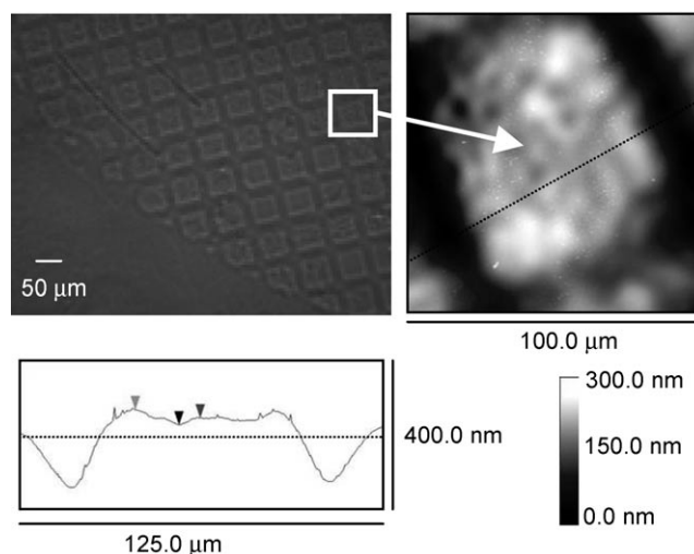
Figure 6. Imaging of a thin film of 1 after imaging and developing. Top left: microscope image; top right: tapping-mode AFM image of the area shown in the inset; bottom left: height profile.
