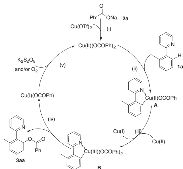
Scheme 3. Plausible mechanism.
