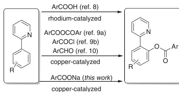
Scheme 1. ortho -Benzoxylation of 2-arylpyridine.
