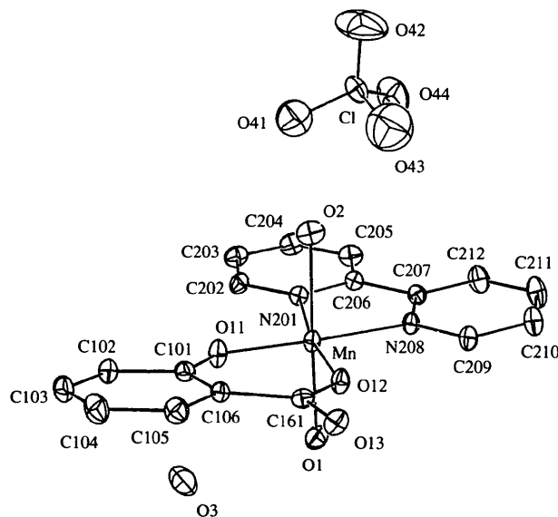
Fig. 1. The asymmetric unit showing 50% probability displacement ellipsoids. H atoms are omitted for clarity.
