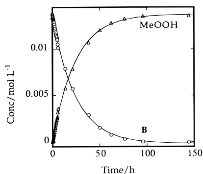
Figure 4. ^1\text{H} -NMR data for the conversion of \text{CH}_3\text{OOH} from B in \text{CD}_3\text{CN} . Conditions: [\text{MTO}]_0 = 14 \text{ mM} , [\text{H}_2\text{O}_2]_0 = 0.75 \text{ M} , [\text{H}_2\text{O}]_0 = 2.6 \text{ M} ; 25^\circ\text{C} .
