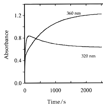
Figure 1. Absorbance-time profiles of the \text{CH}_3\text{ReO}_3 (1.0 mM)- \text{H}_2\text{O}_2 system in \text{CH}_3\text{CN} containing 2.0 M \text{H}_2\text{O} at 25^\circ\text{C} . Data are shown with 36 mM \text{H}_2\text{O}_2 at 320 nm, the maximum for A , and with 100 mM \text{H}_2\text{O}_2 at 360 nm, the maximum for B .
