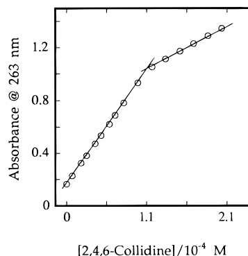
Figure 3. A spectrophotometric titration with 0.012 M 2,4,6-collidine solution in \text{CH}_3\text{CN} . The perhenic acid was titrated in a spent solution that initially contained 1.0 mM \text{CH}_3\text{OREO}_3 and 0.088 M \text{H}_2\text{O}_2 , and which was diluted 8-fold before the titration.
