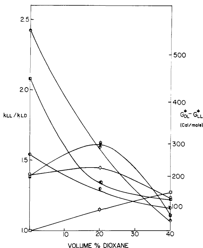
Figure 2. Effect of dioxane addition on the stereoselectivity of bromide displacement from methyl \alpha -bromophenylacetate by tyrosine ethyl ester ( \square ) and the following amide derivatives: amide ( \bullet ), dimethylamide ( \circ ), methyl ester ( \blacksquare ), ethyl ester ( \blacksquare ), isopropyl ester ( \diamond ).
