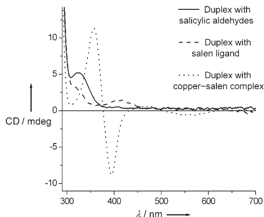
Figure 8. Circular dichroism spectra of 9-L 2 -a/b , [ 9-L 2 -a/b +en], and [ 9-L 2 -a/b +en+Cu] (30 \mu M DNA, 1 mM en, 30 \mu M CuSO 4 , 100 mM NH 4 OAc, pH 8).
