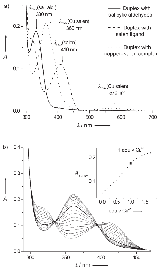
Figure 7. a) Electronic absorption bands of duplexes 9\text{-L}^2\text{-a/b} , [9\text{-L}^2\text{-a/b+en}] , and [9\text{-L}^2\text{-a/b+en+Cu}] ; b) Titration of [9\text{-L}^2\text{-a/b+en}] ( 30\text{ }\mu\text{M} DNA, 1\text{ mM} en, 100\text{ mM} \text{NH}_4\text{OAc}_{(\text{aq})} , pH 8) with \text{Cu}^{2+} in steps of 0.1 equiv; thick line: 1.0 equiv \text{Cu}^{2+} ; inset: plot of \text{Abs}_{360} against the ratio [\text{Cu}^{2+}]/[9\text{-L}^2\text{-a/b+en}] .
