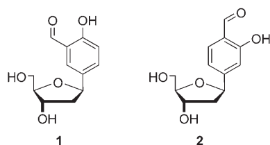
Figure 2. Salicylic aldehyde nucleosides 1 and 2 used to prepare the salen complexes in the DNA strands described in this study.
