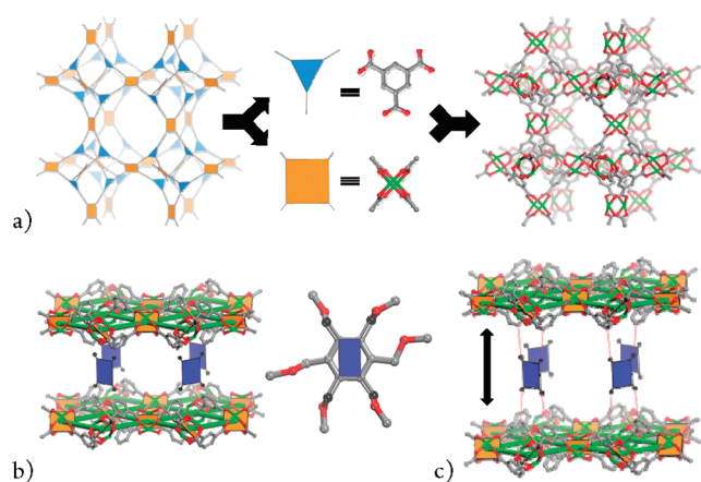
Figure 1. (a) Substitution of the vertex figures in the augmented tbo network, tbo-a , with analogous chemical entities results in a tbo-MOF . (b) tbo-MOFs can be targeted from sql SBLs (green) linked by 4-connected core pillars (blue), which can be functionalized. (c) Extension of the ligand between the core (blue) and the BDC results in a greater distance between the SBLs and increased confined space.
