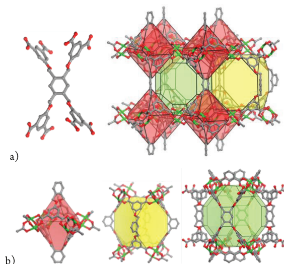
Figure 2. (a) (left) L1 ligand with tetraisophthalate groups connected via alkoxy links to a 4-connected benzene core. (right) Representative section of the crystal structure of 1 showing the polyhedral cages. (b) Three types of polyhedral cage in 1 : truncated tetrahedron (red), truncated cube (yellow), and truncated cuboctahedron (green).
