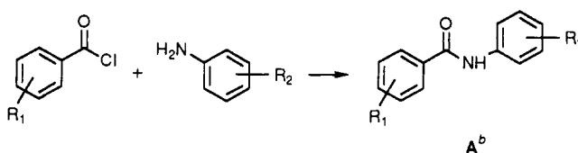
Scheme I. Synthesis of Compounds 1–47 of Table I step 1
