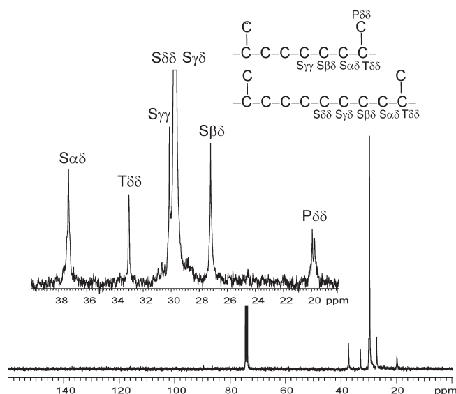
Figure 5. ^{13}\text{C} NMR spectrum of poly(ethylene- co -propylene) (with nearly 7 mol % incorporation of propene) obtained with the 8/d-MAO system catalyst.
