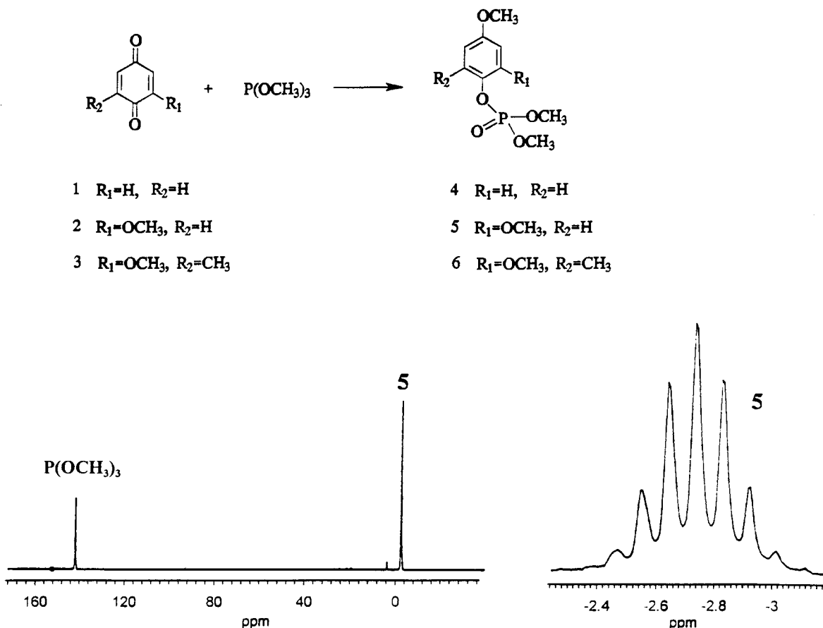
Figure 1. Reaction of p -benzoquinones with trimethyl phosphite and 31 P NMR spectra of compound 5. Its proton-coupled spectrum gives seven lines (right).
