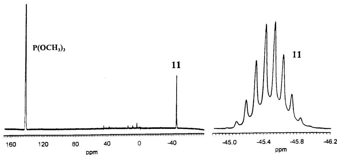
Figure 2. Reactions of o -benzoquinones with trimethyl phosphite and ^{31}\text{P} NMR spectra of compound 11 . Its proton-coupled spectrum gives eight well-resolved and two very weak lines (right).
