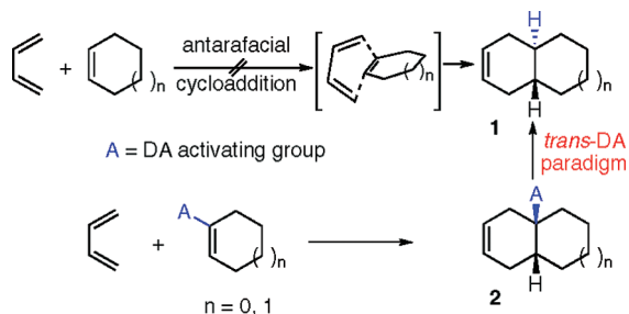
Scheme 1. Trans -Diels–Alder Paradigm
