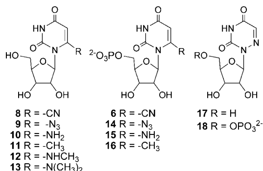
Chart 2. Structures of C6-Uridine Derivatives
