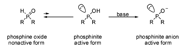
Scheme 1. The Strategy for the Activation of Phosphine Oxides
