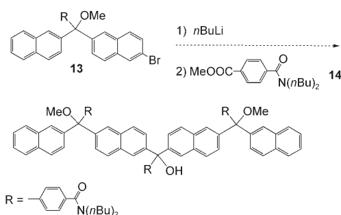
Scheme 6. Failed synthesis of 1,1'-tetramer LON precursor.
