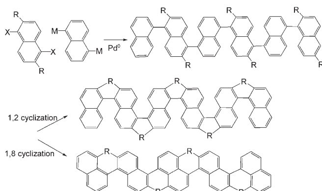
Scheme 2. Difficulties with applying conventional strategy to the synthesis of LONs.
