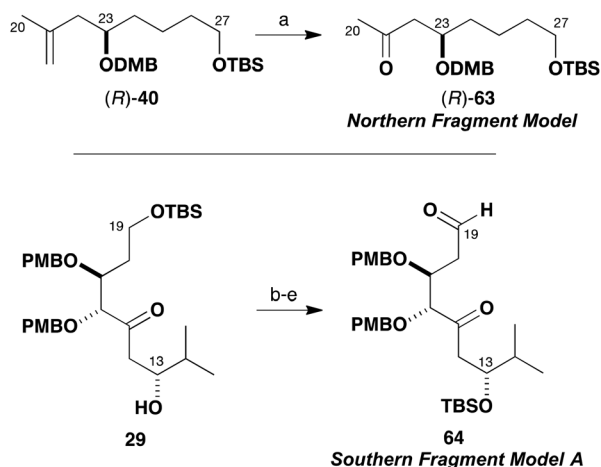
Scheme 13 Preparation of model fragments (R)-63 and 64. Reagents and conditions: (a) \text{OsO}_4 , N -morpholine- N -oxide, \text{THF-H}_2\text{O} ; \text{NaIO}_4\text{-SiO}_2 , 86%; (b) TBSOTf, 2,6-lutidine, \text{CH}_2\text{Cl}_2 , -78^\circ\text{C} , 95%; (c) \text{NaBH}_4 , MeOH, 99%; (d) PPTS, MeOH, 85%; (e) (\text{COCl})_2 , DMSO, \text{CH}_2\text{Cl}_2 , -78^\circ\text{C} ; \text{Et}_3\text{N} , 93%.
