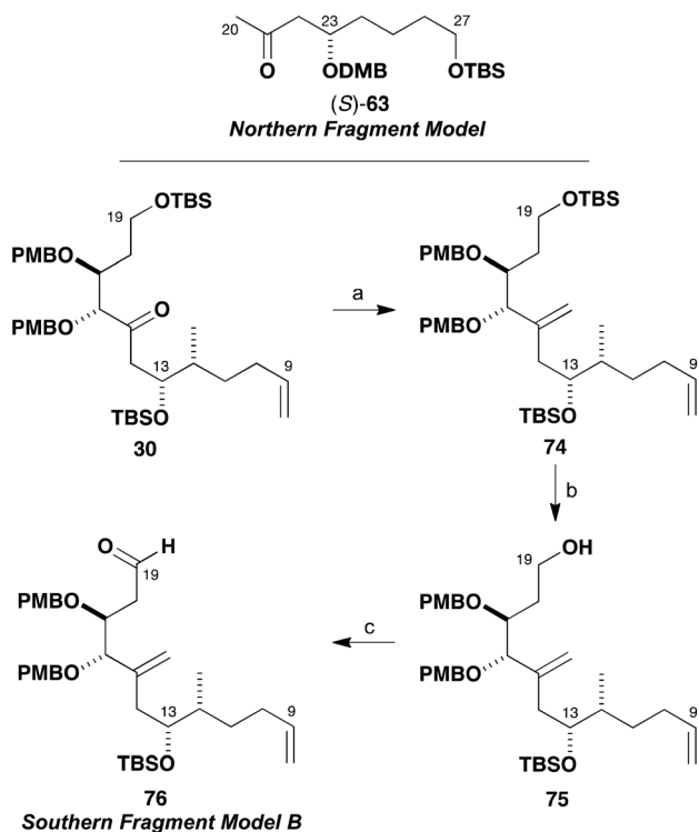
Scheme 17 Preparation of aldehyde 76. Reagents and conditions: (a) Nysted reagent (cyclo-dibromodi- \mu -methylene[ \mu -(tetrahydrofuran)]-triazinc), TiCl 4 , THF, 94% or PbI 2 , CH 2 Cl 2 , Zn, THF, 74%; (b) HF·pyr, pyr, THF, 96%; (c) DMP, NaHCO 3 , CH 2 Cl 2 , 95%.
