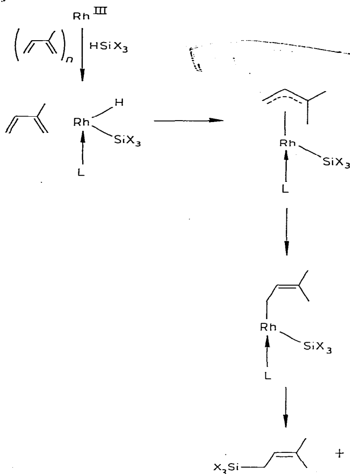
Fig. 2. Proposed mechanism for the hydrosilylation of isoprene using rhodium(III).
