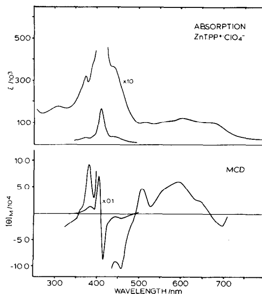
Fig. 4. Absorption and MCD spectra of [\text{ZnTPP}]^{+\bullet}\text{ClO}_4^- , perchloro( \alpha,\beta,\gamma,\delta -tetraphenylporphyrinato)zinc(II) in \text{CH}_2\text{Cl}_2 .
