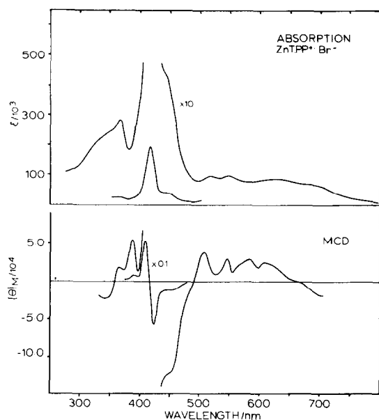
Fig. 3. Absorption and MCD spectra of [\text{ZnTPP}]^{+\bullet}\text{Br}^- , bromo( \alpha,\beta,\gamma,\delta -tetraphenylporphyrinato)zinc(II) in \text{CH}_2\text{Cl}_2 .
