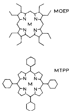
Fig. 1. Molecular geometry of (octaethylporphyrinato)metal(II) and (α,β,γ,δ-tetraphenylporphyrinato)metal(II).
