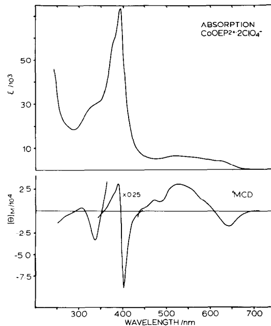
Fig. 11. Absorption and MCD spectra of, [\text{Co(III)OEP}]^{2+} \text{ClO}_4^- , diperchloro(octaethylporphyrinato)cobalt(III) in \text{CH}_2\text{Cl}_2 .
