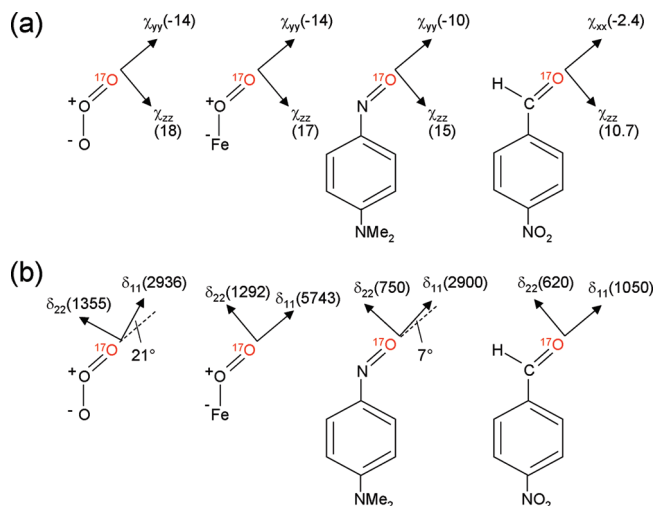
Figure 6. Comparison of ^{17}\text{O} (a) QC and (b) CS tensor orientations in several related \text{X}=\text{O} ( \text{X}=\text{O}, \text{N}, \text{C} ) functional groups. Actual values of the individual tensor components (CS in ppm and QC in MHz) are given in the parentheses. From left to right: ozone, an oxyheme model, NODMA, and p -nitrobenzaldehyde. Only one of the resonance structures is shown for ozone and the oxyheme model to emphasize chemical bonding similarity for the terminal oxygen.
