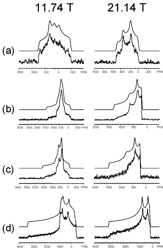
Figure 3. Experimental (lower trace) and simulated (upper trace) ^{17}\text{O} NMR spectra for stationary powder samples of (a) ^{17}\text{O} ]NODMA·HCl, (b) \text{ZnCl}_2(^{17}\text{O})\text{NODMA}_2 , (c) \text{SnCl}_2\text{Me}_2(^{17}\text{O})\text{NODMA}_2 , and (d) ^{17}\text{O} ]NODMA obtained at 11.74 T (left column) and 21.14 T (right column). Detailed experimental parameters are given below. For data collected at 11.74 T: (a) 6912 transients, 10 s recycle time; (b) 5198 transients, 10 s recycle time; (c) 123602 transients, 1 s recycle time; (d) 35384 transients, 2 s recycle time. For data collected at 21.14 T: (a) 6563 transients, 2 s recycle time; (b) 30578 transients, 2 s recycle time; (c) 35204 transients, 2 s recycle time; (d) 12631 transients, 2 s recycle time.
