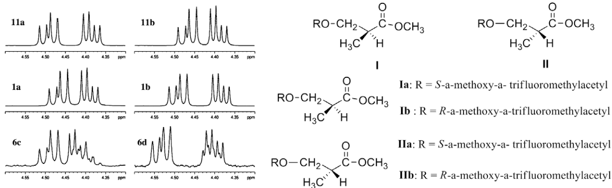
Fig. 1. 1 H NMR signals (400 MHz; CDCl 3 ) due to the methylene protons at C-3 for compounds Ia, IIa, Ib, and IIb.
