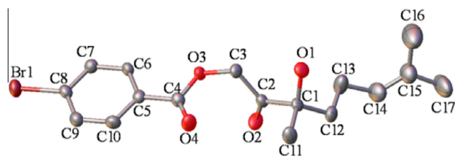
Figure 1. X-Ray crystallographic structure of (R)-8 (CCDC 958550).
