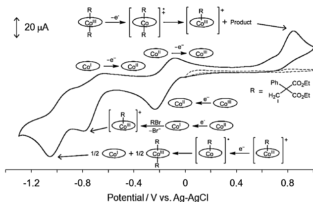
Figure 2. Cyclic voltammograms of 2 (4.5 mM) in the presence of an excess of 3 (10 mM) and in DMF containing n -Bu 4 NPF 6 ( 5.0 \times 10^{-2} M); sweep rate: 100 \text{ mV s}^{-1} ; scan ranges: (solid line) -1.2 to 1.0 \text{ V} vs. Ag–AgCl, (broken line) 0 to 1.0 \text{ V} vs. Ag–AgCl.
