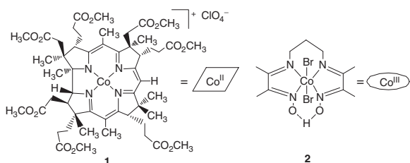
Figure 1. Structures of heptamethyl cobyrinate 1 and [Co III {(DO)(DOH)pn}Br 2 ] ( 2 ).
