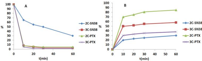
Figure 4. Percent of prodrug remaining (A) and active drug releasing (B) in 1 h of incubation with nitroreductase in presence of NADPH.
