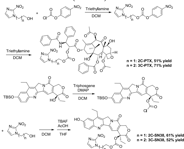
Scheme 1. Synthetic route of prodrugs.
