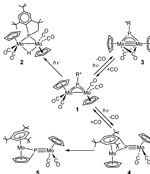
Scheme 1. Photochemical Derivatives of Compound 1 ( \text{R}^* = 2,4,6\text{-C}_6\text{H}_2\text{Bu}_3 )
