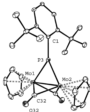
Figure 1. ORTEP diagram of the molecular structure of compound 3 , with hydrogen atoms and one of the t\text{Bu} groups omitted for clarity. Selected bond lengths (Å): Mo(1)–Mo(2) = 2.5322(3), Mo(1)–P(3) = 2.2970(6), Mo(2)–P(3) = 2.3028(5), Mo(1)–C(31) = 2.099(2), Mo(2)–C(31) = 2.141(2), Mo(1)–C(32) = 2.128(2), Mo(2)–C(32) = 2.123(2), P(3)–C(1) = 1.831(2). Bond angles (deg): Mo(1)–P(3)–Mo(2) = 66.8(1), Mo(1)–P(3)–C(1) = 138.8–(1), Mo(2)–P(3)–C(1) = 154.2(1).
