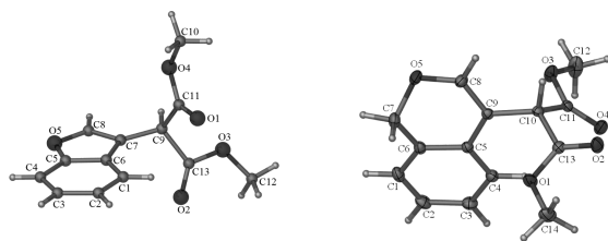
Figure 1. X-ray diffraction studies of 2a (left) and 4k (right).
