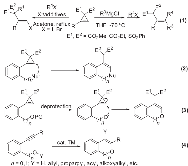
Scheme 1. Ring-Opening Reactions of Cyclopropene Derivatives and the Syntheses of Benzofurans
