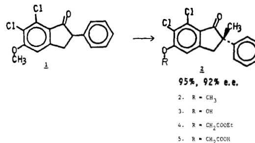
Scheme I
