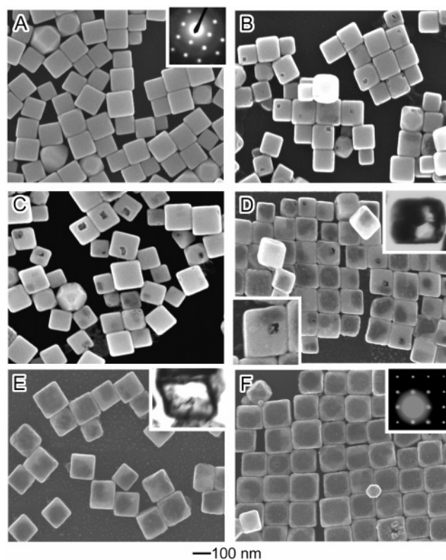
Figure 1. Formation of Au–Ag nanoboxes through a combination of galvanic replacement reaction (between Ag and HAuCl 4 ) and alloying (between Au and Ag). The SEM images were taken from silver nanocubes (A) before and (B–F) after they had reacted with different volumes of 1 mM HAuCl 4 solution: (B) 0.05, (C) 0.10, (D) 0.30, (E) 0.50, and (F) 0.75 mL. The formation of hollow structures was confirmed by TEM studies on the microtomed samples (the insets at the upper right-hand corners of panels D and E). The formation of slightly truncated corners for the nanoboxes shown in F implies the initiation of dealloying.
