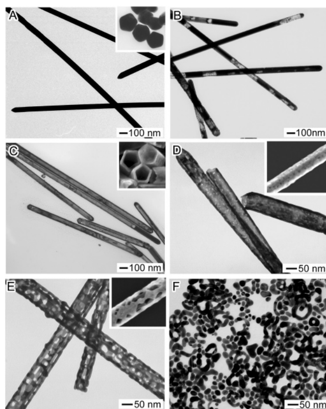
Figure 7. TEM images taken from silver nanowires (A) before and (B–F) after they had reacted with different volumes of 1 mM \text{HAuCl}_4 solution: (B) 0.3, (C) 0.6, (D) 1.5, (E) 2.3, and (F) 3.0 mL. The inset of A shows TEM image taken from the microtomed sample of silver nanowires. The insets of C–E are SEM images of the corresponding products.
