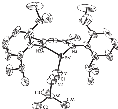
Figure 1. Molecular structure of 2 . Thermal ellipsoids are shown at 50% probability. H atoms are omitted for clarity reasons. Selected bond lengths [Å] and angles [deg]: \text{Sn1-N1} 2.121(7), \text{N1-C1} 1.124(10), \text{C1-N2} 1.239(11), \text{N2-Si1} 1.718(7), \text{Sn1-N3} 2.169(3); \text{Sn1-N1-C1} 152.5(8), \text{N1-C1-N2} 178.6(10), \text{C1-N2-Si1} 136.2(7), \text{N1-Sn1-N3} 90.35(18), \text{N3-Sn1-N3A} 86.5(2).
