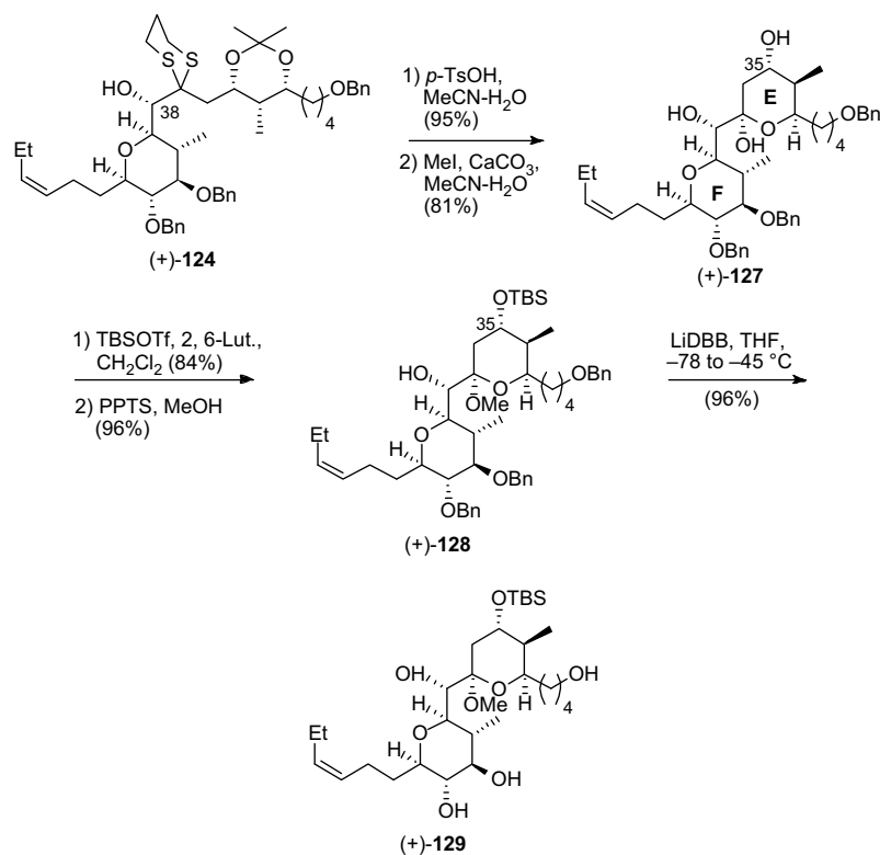
Scheme 41.
