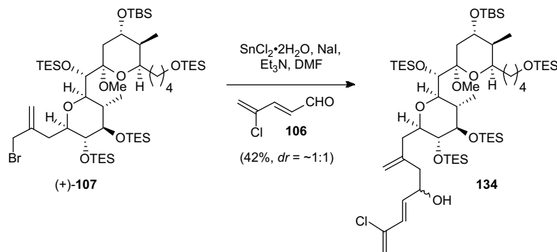
Scheme 43.
