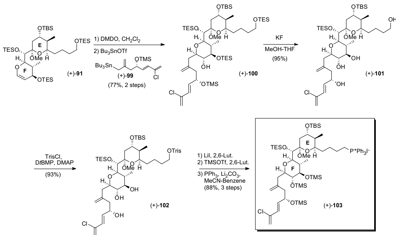
Scheme 34.
