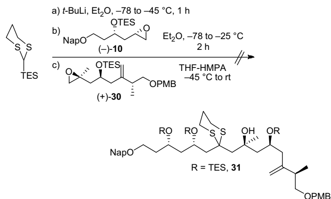
Scheme 9.
