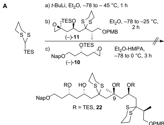
Scheme 6A.
