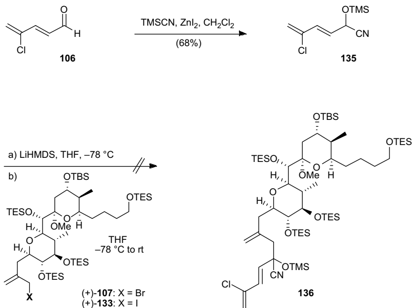
Scheme 44.
