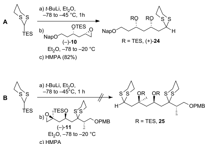
Scheme 7.
