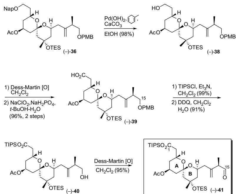
Scheme 13.
