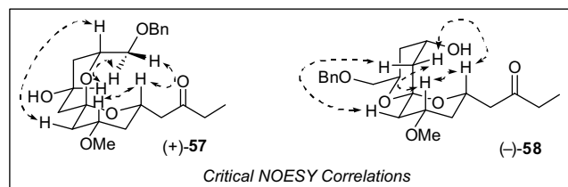
Figure 2. Relevant NOESY data for (+)-57 and (-)-58.
