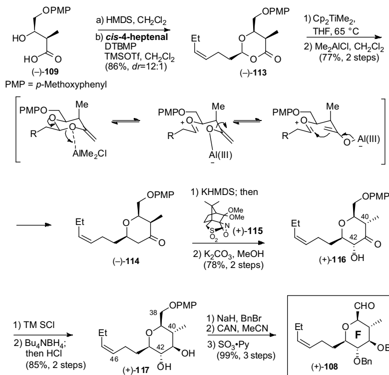
Scheme 37.
