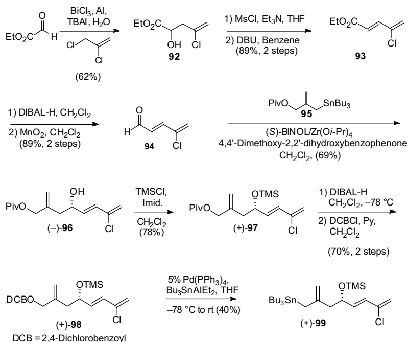
Scheme 33.
