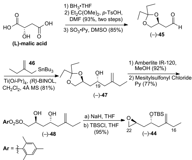
Scheme 15.
