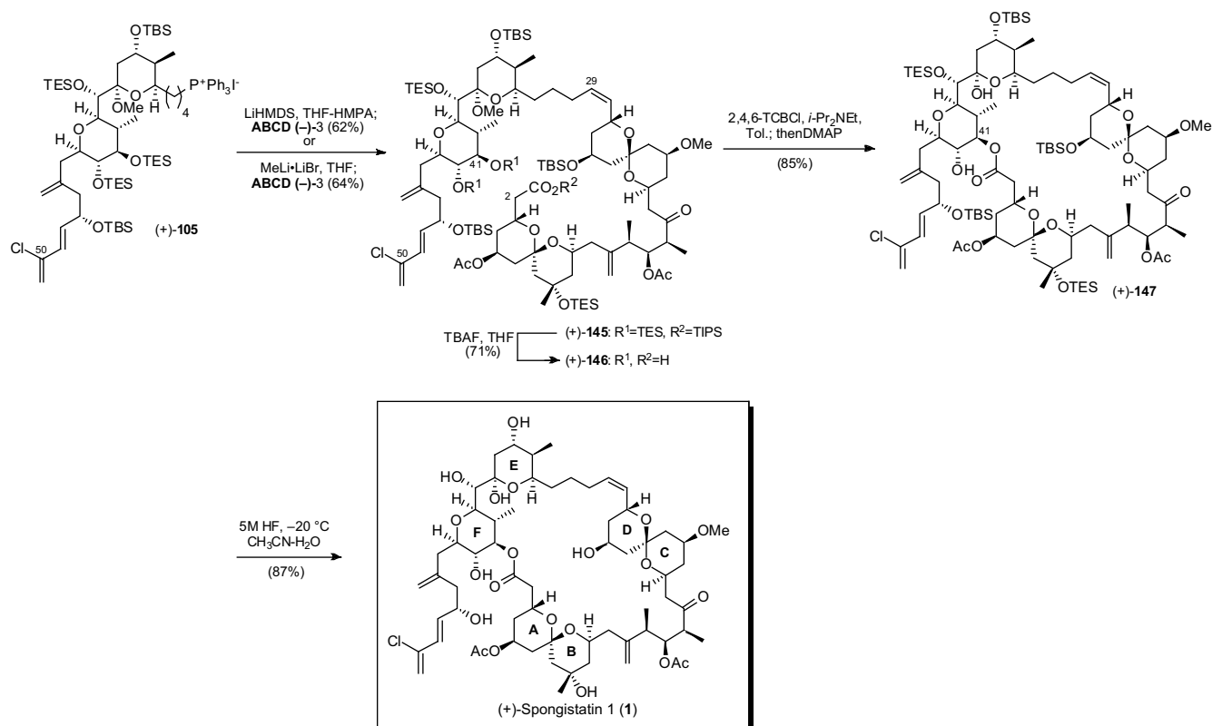
Scheme 47.
