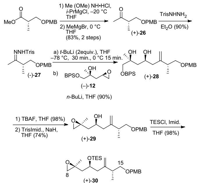
Scheme 8.
