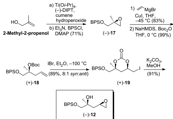
Scheme 4.
