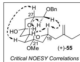
Figure 1. Critical NOESY NMR correlations for spiroketal (+)-55.
