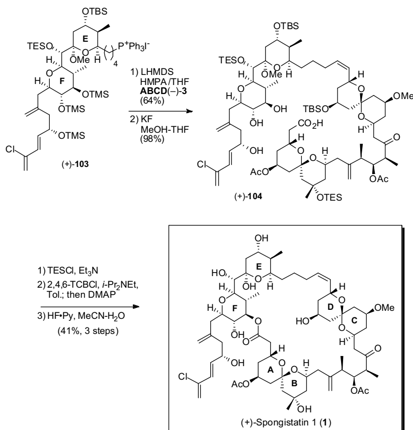
Scheme 35.
