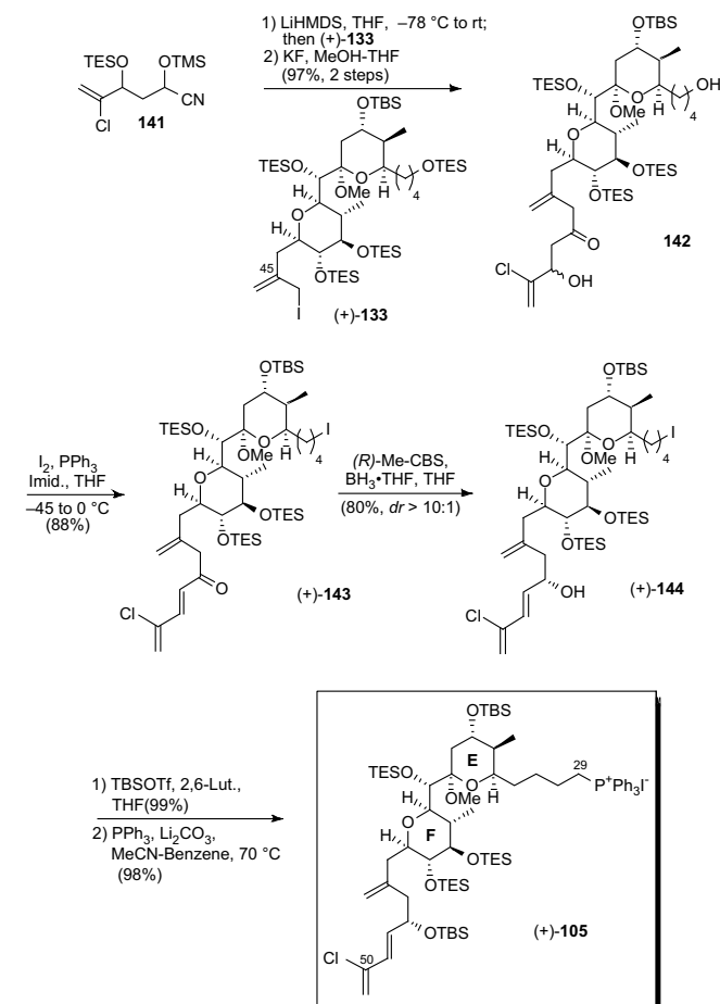
Scheme 46.
