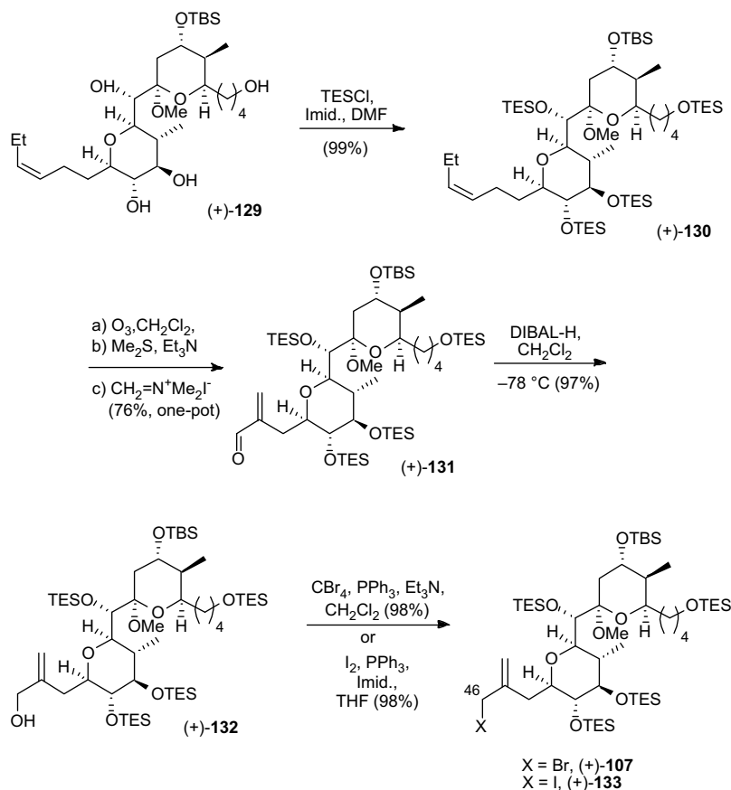
Scheme 42.
