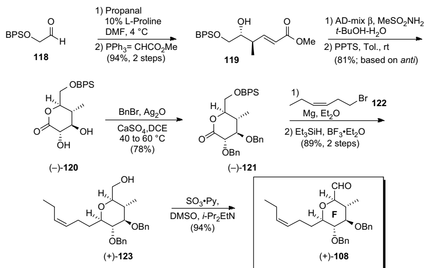
Scheme 39.
