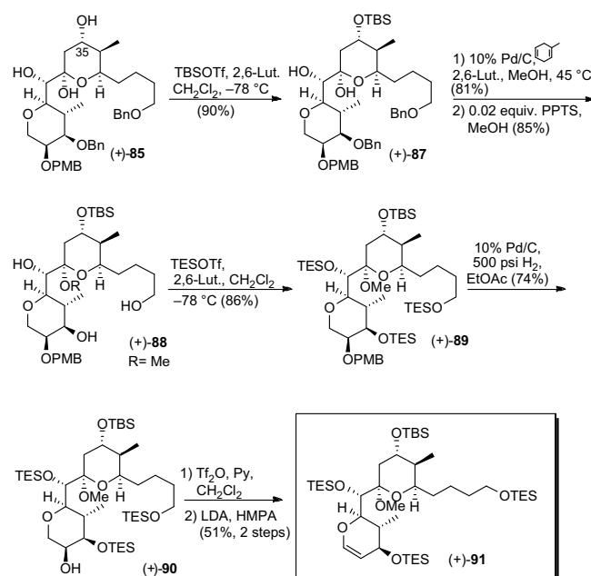
Scheme 32.
