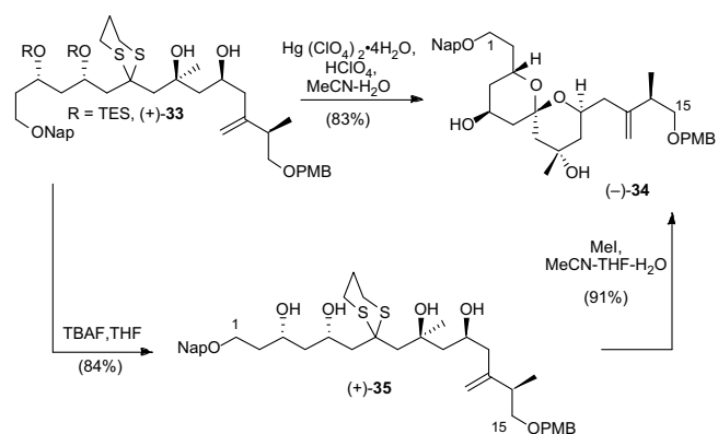
Scheme 11.
