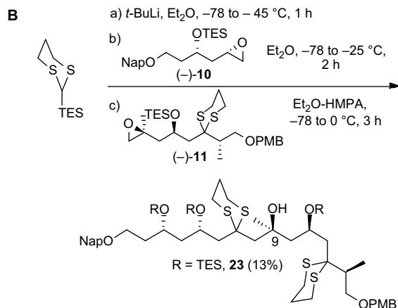
Scheme 6B.
