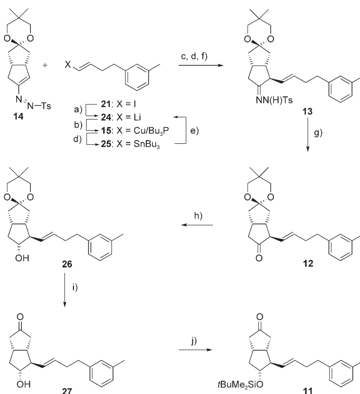
Scheme 4. Conjugate addition of the alkenylcopper compound 15 to azoalkene 14 . a) 21 (2 equiv), n\text{BuLi} (2 equiv), THF, -78^\circ\text{C} , 3 h; b) \text{CuI} (2 equiv), \text{Bu}_3\text{P} (5.2 equiv), THF, -78^\circ\text{C} , 10 min; c) 14 (1 equiv), THF, -78^\circ\text{C} , 45 min; d) \text{Bu}_3\text{SnCl} (2.9 equiv); e) t\text{BuLi} , THF, -78^\circ\text{C} ; f) aqueous \text{NH}_4\text{Cl} ; g) cyclohexene (7.4 equiv), (\text{PhSeO})_2\text{O} , THF, RT; h) \text{NaBH}_4 , EtOH, 0^\circ\text{C} ; i) \text{H}_2\text{O} , \text{TsOH} , acetone, RT; j) t\text{BuMe}_2\text{SiCl} , imidazole, DMF, RT.
