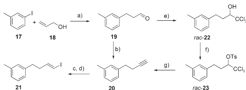
Scheme 3. Synthesis of the alkenyl iodide 21 . a) \text{Pd}(\text{OAc})_2 , \text{NaHCO}_3 , \text{Bu}_4\text{NCl} , DMF, 30^\circ\text{C} ; b) (\text{CH}_3)_3\text{SiCHN}_2 , n\text{BuLi} , THF, -78^\circ\text{C} to RT; c) \text{Cp}_2\text{Zr}(\text{H})\text{Cl} , \text{CH}_2\text{Cl}_2 , RT; d) \text{I}_2 , \text{CH}_2\text{Cl}_2 , RT; e) \text{Cl}_3\text{CCO}_2\text{H}/\text{Cl}_3\text{CCO}_2\text{Na} , DMF, RT; f) \text{TsCl} , \text{NEt}_3 , DABCO, \text{CH}_2\text{Cl}_2 , RT; g) \text{MeLi} , THF, -78^\circ\text{C} to RT. Cp=cyclopentadienyl; DABCO=1,4-diazabicyclo[2.2.2]octane.
