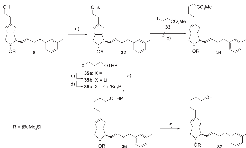
Scheme 7. Formal synthesis of 15-deoxy-TIC ( 7a ). a) TsCl, NEt 3 , DABCO, CH 2 Cl 2 , RT; b) Zn (1 equiv), dibromomethane (0.036 equiv), ClSiMe 3 (0.036 equiv); 33 (0.97 equiv), THF; CuCN (0.80 equiv), LiCl (1.7 equiv), THF; 32 ; c) t BuLi (2 equiv), Et 2 O, n -pentane, −78°C, 1 h; d) CuI (1 equiv), Bu 3 P (2.6 equiv), Et 2 O, −78 to −40°C; e) 32 (0.25 equiv), Et 2 O, −40 to 0°C, 2 h; f) MgBr 2 , Et 2 O. THP = tetrahydropyranyl.
