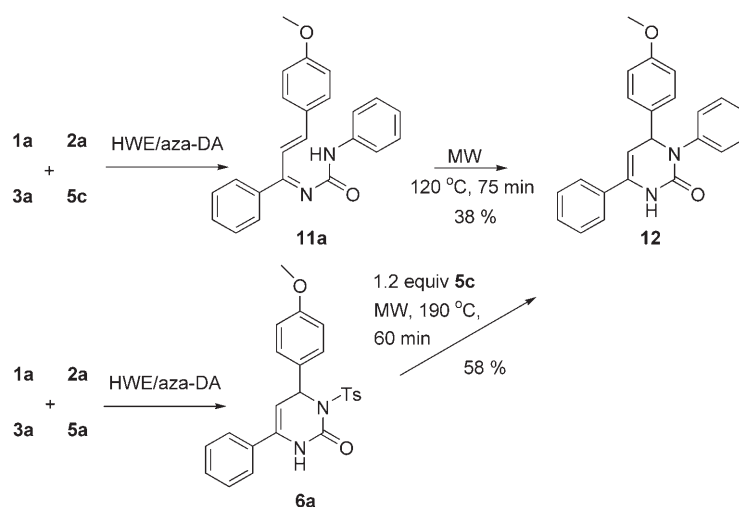
Scheme 5. Synthesis of DHPMs 12 with less electron-withdrawing \text{R}^4 substituents.
