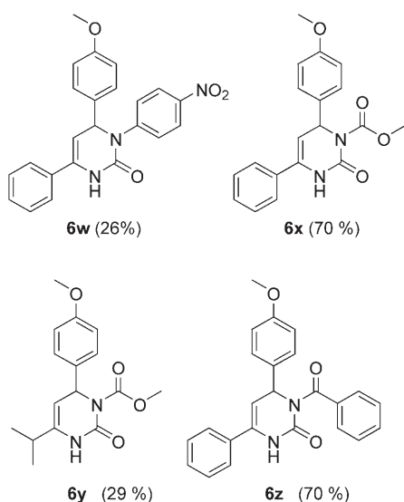
Scheme 4. DHPMs 6 formed with various isocyanates 5 .
