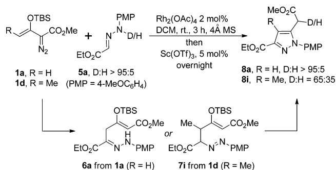
Scheme 4. Labeling Experiments Define Outcome of Vinylogous Addition Step
