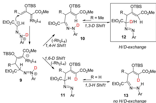
Scheme 5. Possible Pathways for Deuterium Retention/Loss
