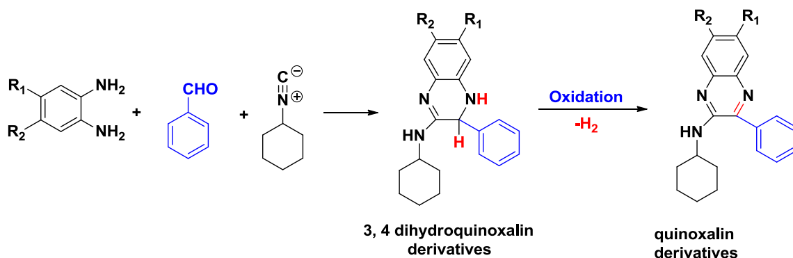
Scheme 1 Aldehyde's hydrogen involves in reaction path way [11, 12] and quinoxaline derivative is formed
