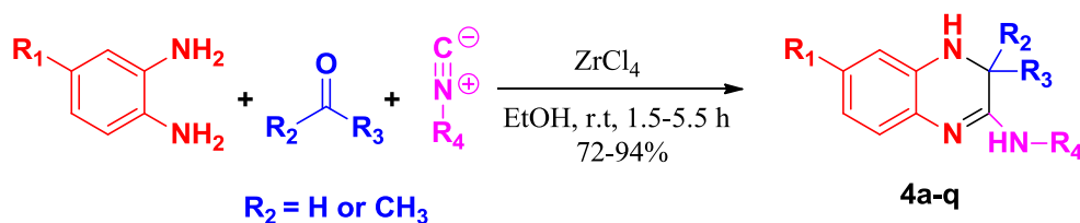
Scheme 2 Synthesis of 3,4-dihydroquinoxalin-2-amine derivatives 4
