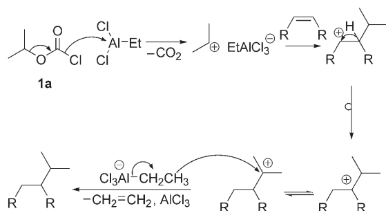
Scheme 1. Mechanism of the hydroalkylation of alkenes with isopropyl chloroformate ( 1a ) induced by ethylaluminum sesquichloride. R = alkyl.
