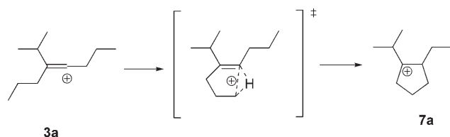
Scheme 4. Concerted intramolecular insertion of vinyl cation 3a into a primary C–H bond to give the cyclopentyl carbenium ion 7a .
