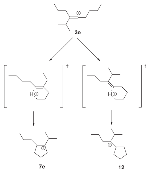
Scheme 5. Model reaction of vinyl cation 3e by endo- and exocyclic pathways to give the cyclopentyl cations 7e and 12 .
