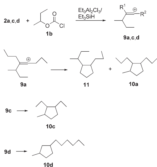
Scheme 3. Reaction of alkynes 2a,c,d with 1b in the presence of Et 3 Al 2 Cl 3 /Et 3 SiH proceeding via vinyl cations 9a,c,d to give the products of a hydroalkylating cyclization 10a,c,d and 11 . Cyclopentanes 10a and 11 are formed in a ratio of 1:3 via vinyl cation 9a . The cyclopentanes were obtained as mixtures of diastereomers. For R 1 , R 2 , see Scheme 2.
