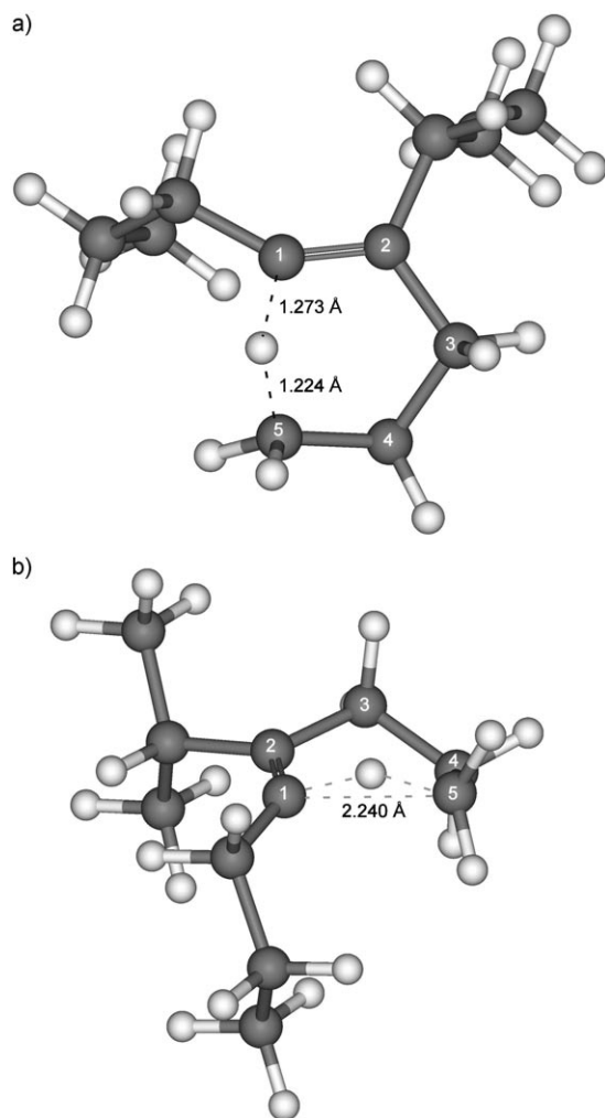
Figure 1. Transition state for the concerted formation of cyclopentyl cation 7a from vinyl cation 3a . Relevant C–H and C–C distances are given. a) View of the forming cyclopentane ring in the plane. b) The view of the forming cyclopentane ring perpendicular to the plane reveals a boatlike orientation; carbon atoms 2–4 lie above the C1–H–C5 plane. The C1–H–C5 angle is 127.5°.
