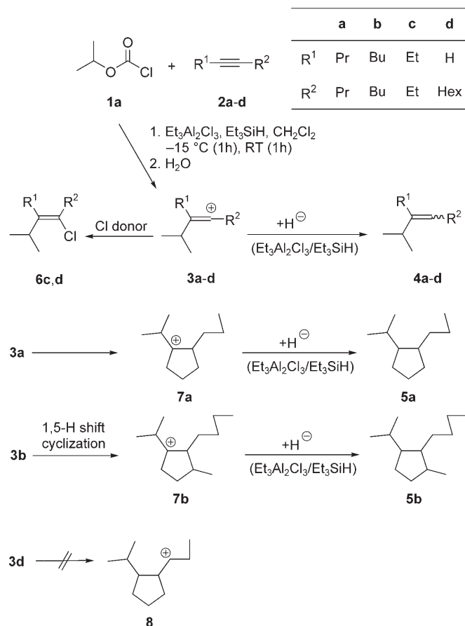
Scheme 2. Reactions of alkynes 2a–d with 1a in the presence of Et 3 Al 2 Cl 3 /Et 3 SiH proceeding via vinyl cations 3a–d . Products 5a,b and 6c,d as well as the side products 4a–d were obtained as mixtures of diastereomers. Products derived from the exocyclic cyclopentyl cation 8 were not observed.
