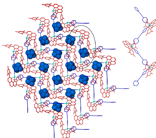
Figure 3. View of the 2D packing arrangement of complex \text{C1}^{(II)} with \text{PF}_6^- anions (shown in a space filling mode) inside the channel. Inset shows the zigzag motif of an individual chain structure. Hydrogen atoms were omitted for clarity. Color code: 1, red; 3, blue; copper, cyan.
