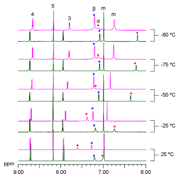
Figure 8. Variable temperature ^1\text{H} NMR spectra (partial spectrum) of \text{C1}^{(\text{I})} and \text{C1S}^{(\text{III})} , all in \text{CD}_2\text{Cl}_2 . Color code: \text{C1}^{(\text{I})} , green; \text{C1S}^{(\text{III})} , pink; \text{py}_\alpha , red stars; \text{py}_\beta , blue stars.
