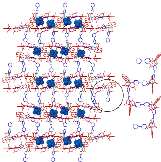
Figure 5. Crystal packing of complex C3 (II) along c axis, with \text{PF}_6^- anions (shown in space filling mode) located in between the 2D layers. Inset shows the twist in the chain structure. Color code: 1, red; 2, blue; copper, cyan. All hydrogen atoms were omitted for clarity.
