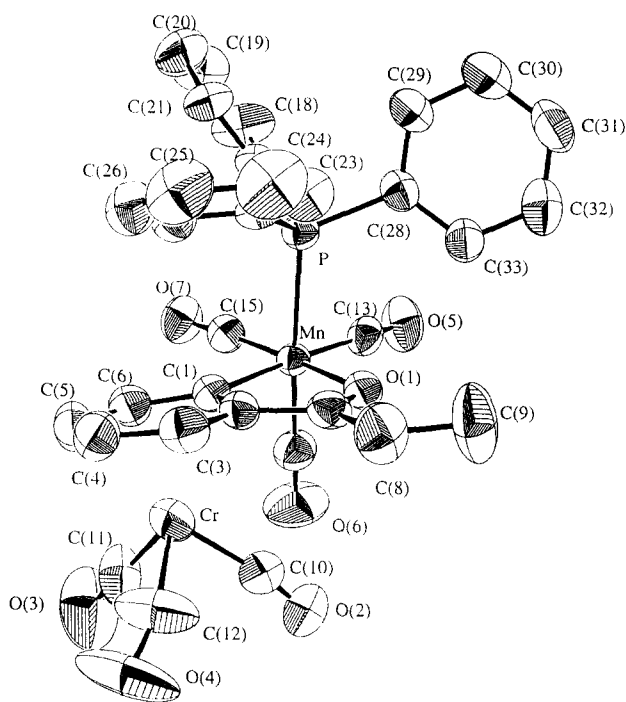
Fig. 5. The atomic arrangement in 29 .
