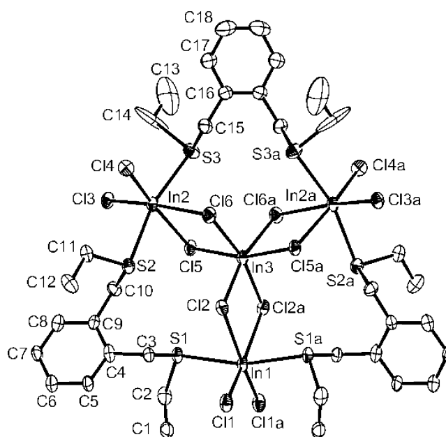
Figure 6. View of the structure of [(\text{InCl}_3)_4\{o\text{-C}_6\text{H}_4(\text{CH}_2\text{SEt})_2\}_3] , 9 , with atom-numbering scheme. Ellipsoids are shown at the 50% probability level, and H atoms are omitted for clarity. Symmetry operation: a = -x, y, 1/2 - z .
