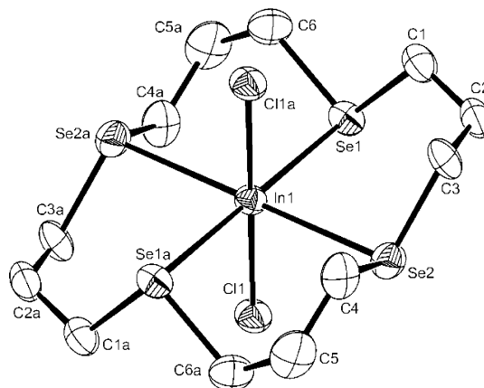
Figure 4. View of the structure of the centrosymmetric cation in 4 with atom-numbering scheme. Ellipsoids are shown at the 40% probability level, and H atoms are omitted for clarity. Symmetry operation: a = -x, 1 - y, 2 - z . Selected bond lengths (Angstroms) and angles (degrees): In1–Cl1 = 2.475(2), In1–Se1 = 2.7189(10), In1–Se2 = 2.7394(11); Cl1–In1–Se1 = 88.04(6), Cl1–In1–Se2 = 88.10(6).
