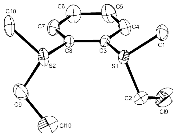
Figure 5. View of the structure of the dication in 6 with atom-numbering scheme. Ellipsoids are shown at the 50% probability level, and H atoms are omitted for clarity. Selected bond lengths (Angstroms) and angles (degrees): S1–C1 = 1.786(8), S1–C2 = 1.820(8), S1–C3 = 1.779(7), S2–C8 = 1.790(7), S2–C9 = 1.821(9), S2–C10 = 1.812(9); C1–S1–C2 = 101.3(4), C1–S1–C3 = 104.9(4), C2–S1–C3 = 103.5(4), C8–S2–C9 = 101.1(4), C8–S2–C10 = 104.0(4), C9–S2–C10 = 100.7(4).
