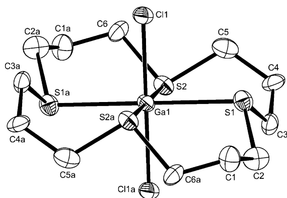
Figure 2. View of the cation in 2 with atom-numbering scheme. Ellipsoids are shown at the 50% probability level, and H atoms are omitted for clarity. Symmetry operation: a = 2 - x, -y, 1 - z .
