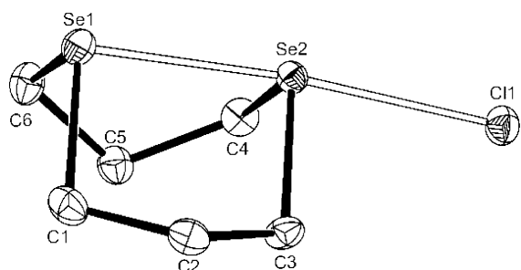
Figure 8. View of the structure of the cation in 12 · \text{CH}_2\text{Cl}_2 with atom-numbering scheme. Ellipsoids are shown at the 50% probability level, and H atoms are omitted for clarity. Selected bond lengths (Angstroms) and angles (degrees): Se2–C11 = 2.5346(6), Se1–C1 = 1.970(2), Se1–C6 = 1.967(2), Se1–Se2 = 2.5229(4), Se2–C3 = 1.981(2), Se2–C4 = 1.978(2); C1–Se1–C6 = 99.66(9), C3–Se2–C4 = 101.93(9), C4–Se2–C11 = 89.39(6), C3–Se2–C11 = 88.09(6), Se1–Se2–C11 = 175.23(2).
