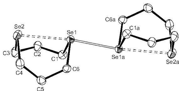
Figure 7. View of the structure of the dimeric cation in 11 with atom-numbering scheme. Ellipsoids are shown at the 50% probability level, and H atoms are omitted for clarity. Symmetry operation: a = -x, -y, -z . Selected bond lengths (Angstroms) and angles (degrees): Se1–C1 = 1.980(3), Se1–C6 = 1.981(3), Se1–Se1a = 2.6662(7), Se1...Se2 = 2.891(1), Se2–C3 = 1.957(3), Se2–C4 = 1.962(3); C1–Se1–C6 = 99.69(13), C3–Se2–C4 = 99.71(15).
