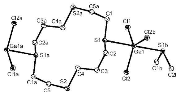
Figure 1. View of the structure of a section of the chain polymer of 1 with atom-numbering scheme. Ellipsoids are shown at the 50% probability level, and H atoms are omitted for clarity. Symmetry operators: a = 1/2 - x, 1/2 - y, -z ; b = 1 - x, y, 1/2 - z .
