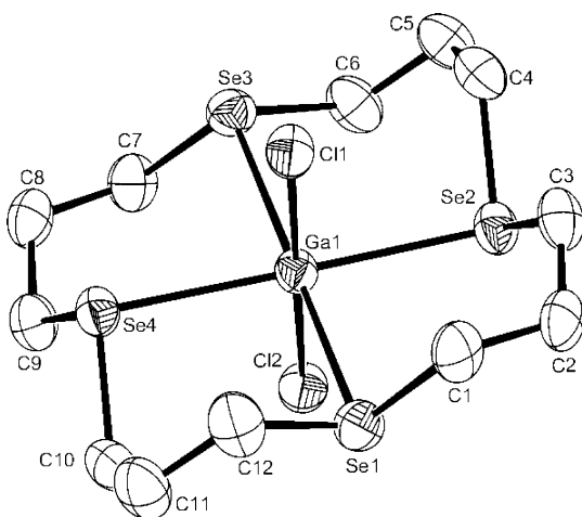
Figure 3. View of the structure of the cation in 3 with atom-numbering scheme. Ellipsoids are shown at the 50% probability level, and H atoms are omitted for clarity.
