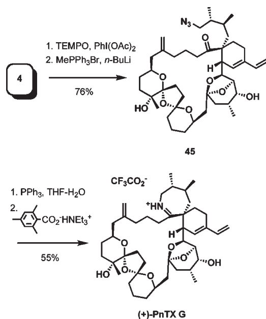
Scheme 9. Total Synthesis of PnTX G
