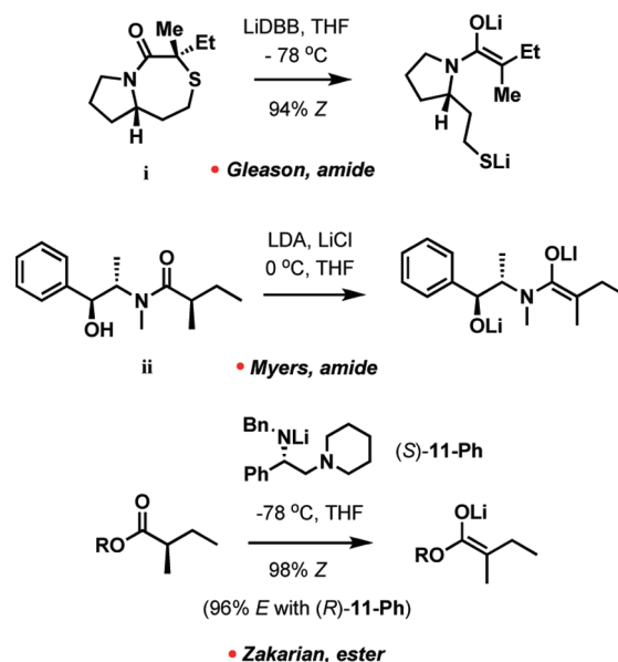
Scheme 3. Examples of Stereoselective Generation of Acyclic \alpha,\alpha -Disubstituted Enolates
