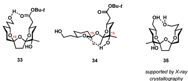
Figure 2. Hydrogen-bonding stabilization in spiroketal intermediates.
