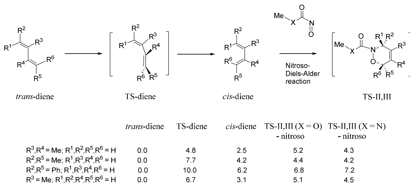
Figure 6. Relative energies (kcal mol -1 ) for computed acyclic diene and nitroso-Diels-Alder model pathways.
