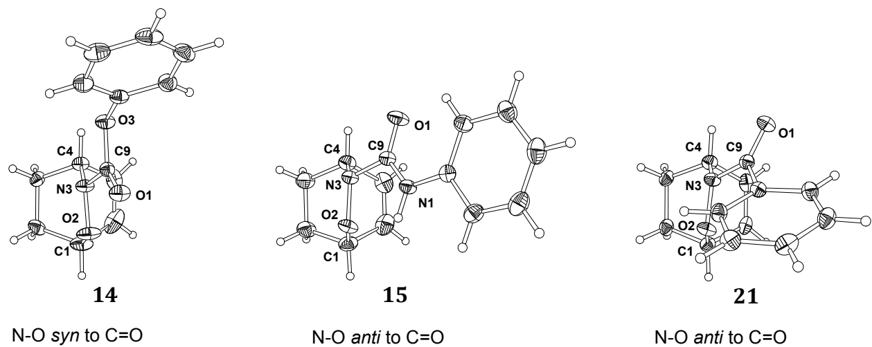
Figure 2. Views of the substituents at N3 with respect to the bicyclic framework in molecular structures of 14 , 15 and 21 .
