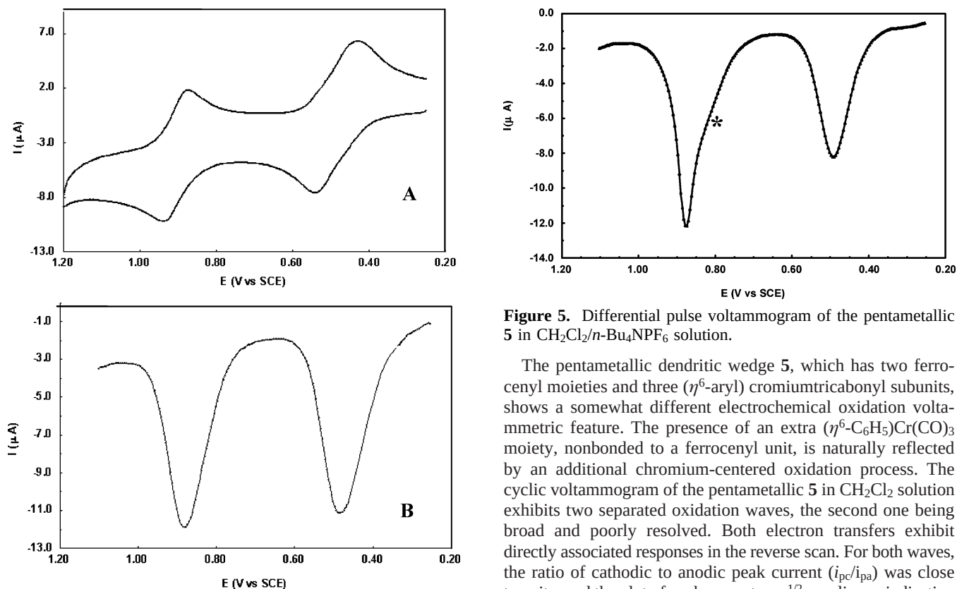
Figure 4. Cyclic voltammogram (A) and differential pulse voltammogram (B) of 7 in \text{CH}_2\text{Cl}_2 solution.
