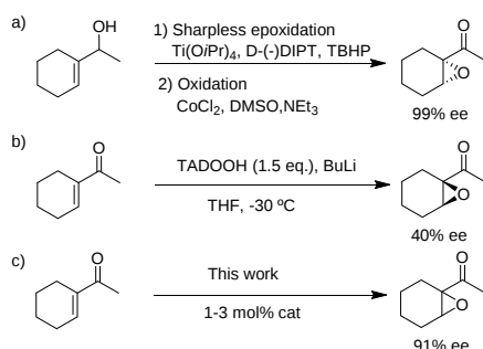
Scheme 1. Examples in the literature for epoxidation of 1-acetyl-1-cyclohexene
