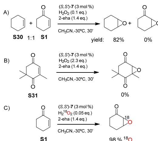
Scheme 2. Mechanistic scenarios for the asymmetric epoxidation of a cyclic enone. A) Nucleophilic Weitz–Scheffer epoxidation mechanism and B) Electro-
