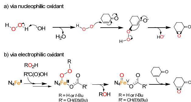
Scheme 2. Mechanistic scenarios for the asymmetric epoxidation of a cyclic enone. A) Nucleophilic Weitz–Scheffer epoxidation mechanism and B) Electro-
