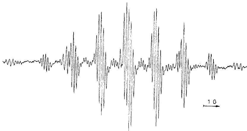
Fig. 2. ESR spectrum of the biphenylene dimer radical cation 1_2^{++} in dichloromethane at 180 K.
