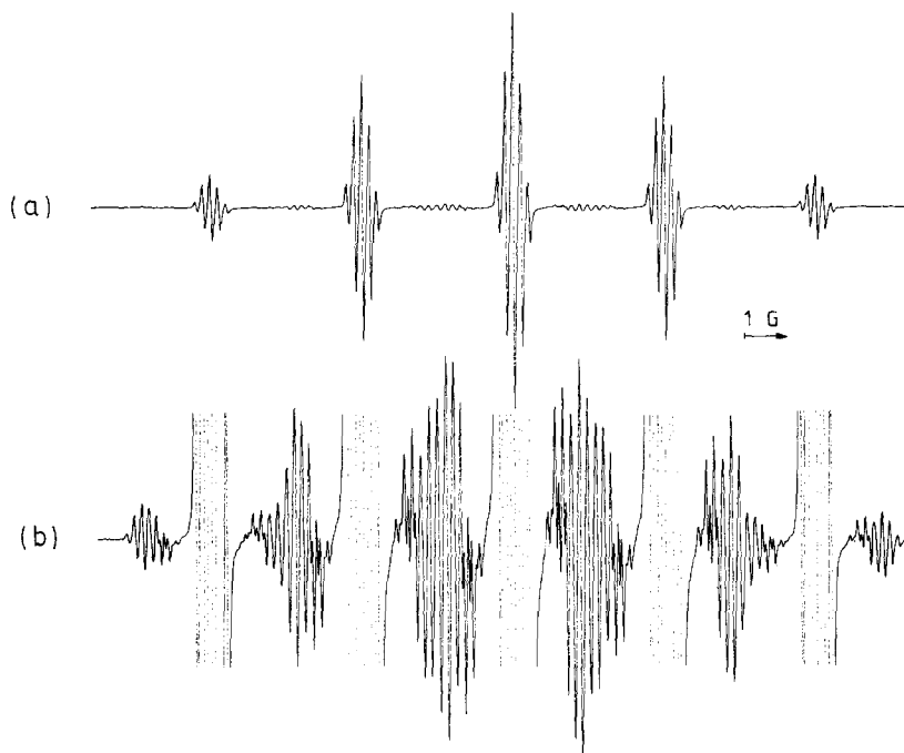
Fig. 1. ESR spectrum (a) of the biphenylene radical cation 1^{++} in trifluoroacetic acid at 260 K, together with, (b), the ^{13}\text{C} satellites.
