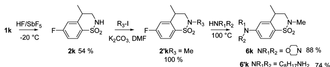
Scheme 2. 4-Aminobenzofused Sultam Synthesis
