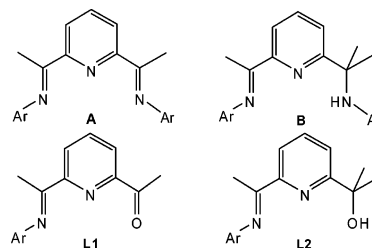
Chart 1. 2,6-Bis(imino)pyridine ( A ), 2-Imino-6-(methylamino)pyridine ( B ), 2-Acetyl-6-iminopyridine ( L1 ), and 2-Imino-6-(methyl alcohol)pyridine ( L2 )
