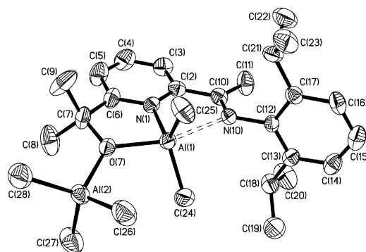
Figure 1. Molecular structure of one (A) of the two independent molecules present in the crystals of 1a (50% probability ellipsoids); hydrogen atoms omitted for clarity. Selected bond lengths (Å) and angles (deg): Al(1)–O(7) 1.907(3), Al(1)–N(1) 1.994(4), Al(1)–C(24) 1.952(5), Al(1)–C(25) 1.959(5), Al(1)···N(10) 2.427(4), Al(2)–O(7) 1.917(3), Al(2)–C(26) 1.984(5), Al(2)–C(27) 1.983(5), Al(2)–C(28) 1.986(5), C(7)–O(7) 1.436(5), C(10)–N(10) 1.288(5), C(24)–Al(1)–C(25) 125.2(3), O(7)–Al(1)···N(10) 152.82(13), O(7)–C(7)–C(8) 110.2(4), O(7)–C(7)–C(9) 109.4(4), O(7)–Al(2)–C(26) 106.2(2), C(26)–Al(2)–C(27) 112.2(3), C(27)–Al(2)–C(28) 111.4(2).
