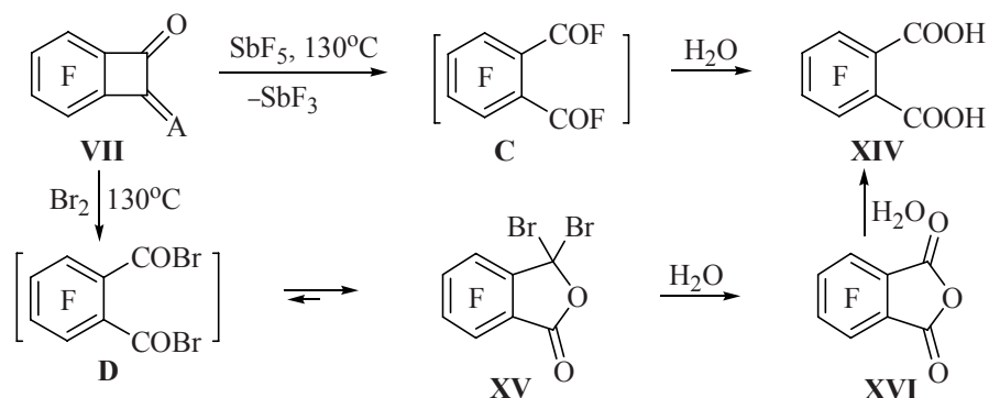
Scheme 3.
