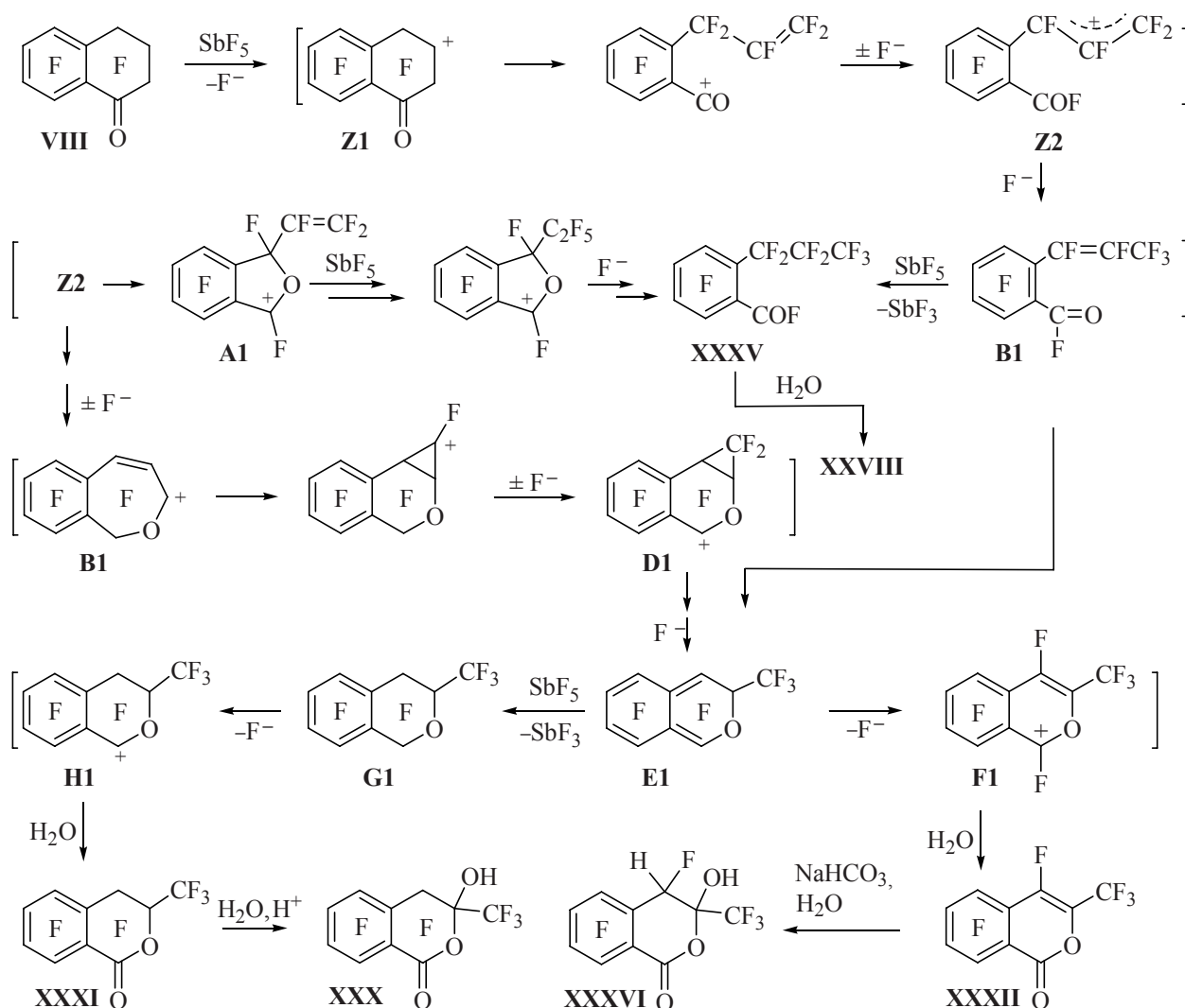
Scheme 11.
