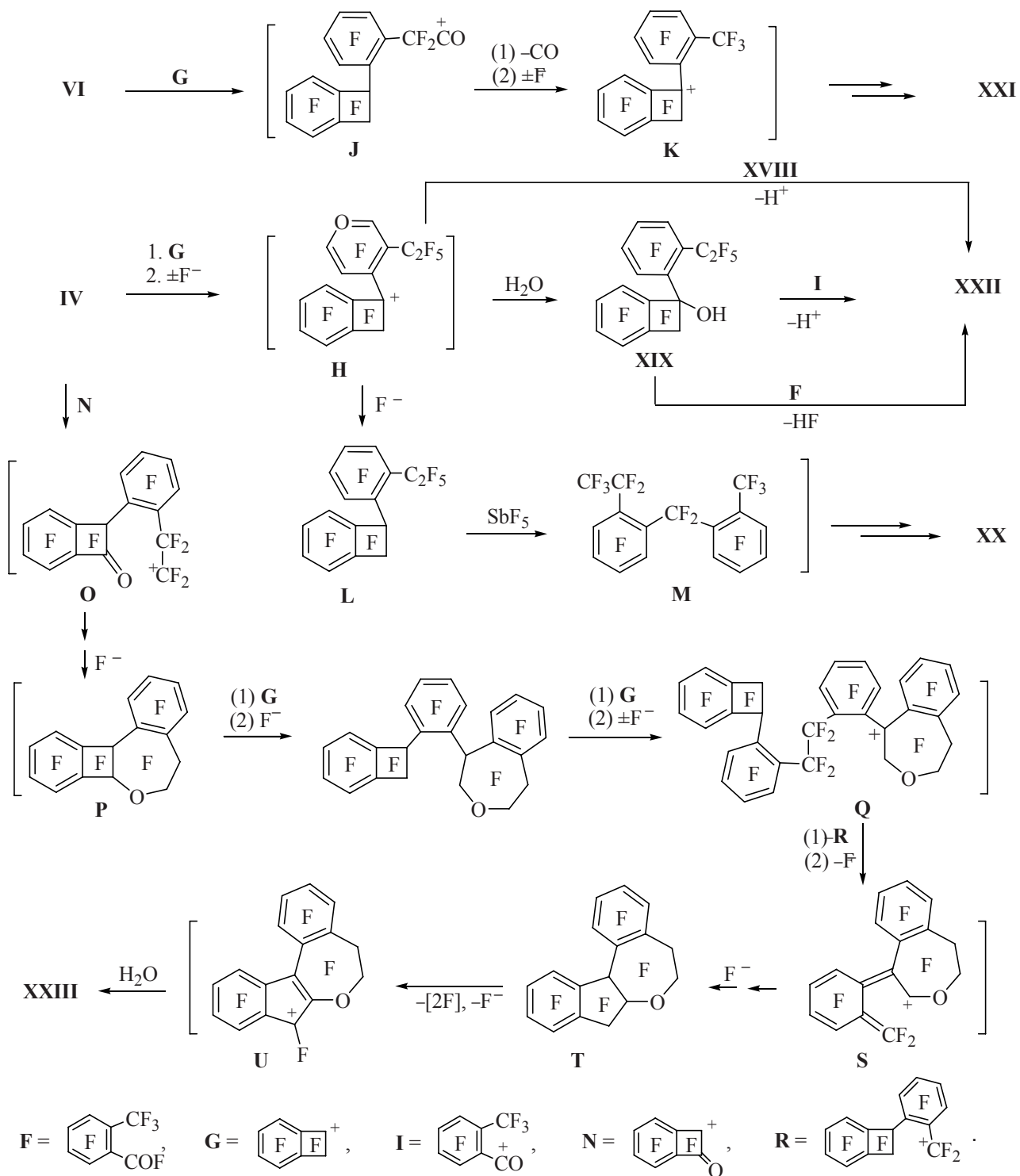
Scheme 7.
