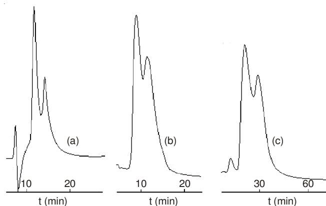
Fig. 4. Enantioseparation chromatograms of racemates. (a): 2-phenyl-1-propanol on uridine column; (b): pindolol on thymidine column; (c): furoin on thymidine column
