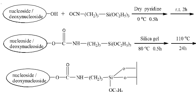
Fig. 2. Scheme of the synthesis of chiral stationary phases
