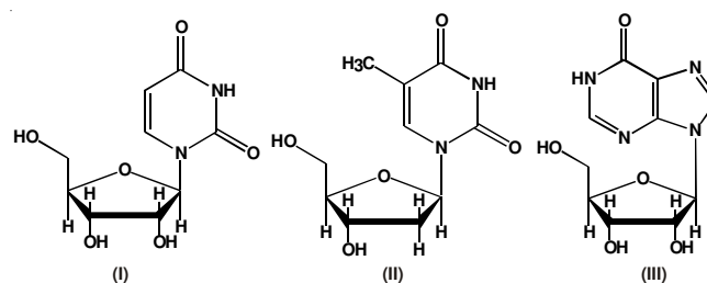
Fig. 1. Structures of uridine(I), thymidine(II) and inosine(III)
