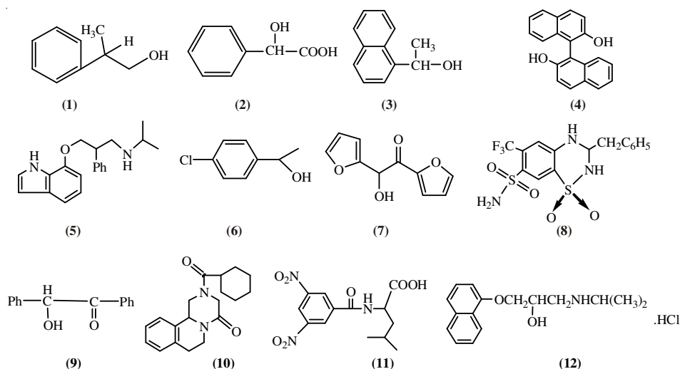
Fig. 3. Molecular structures of chiral compounds
